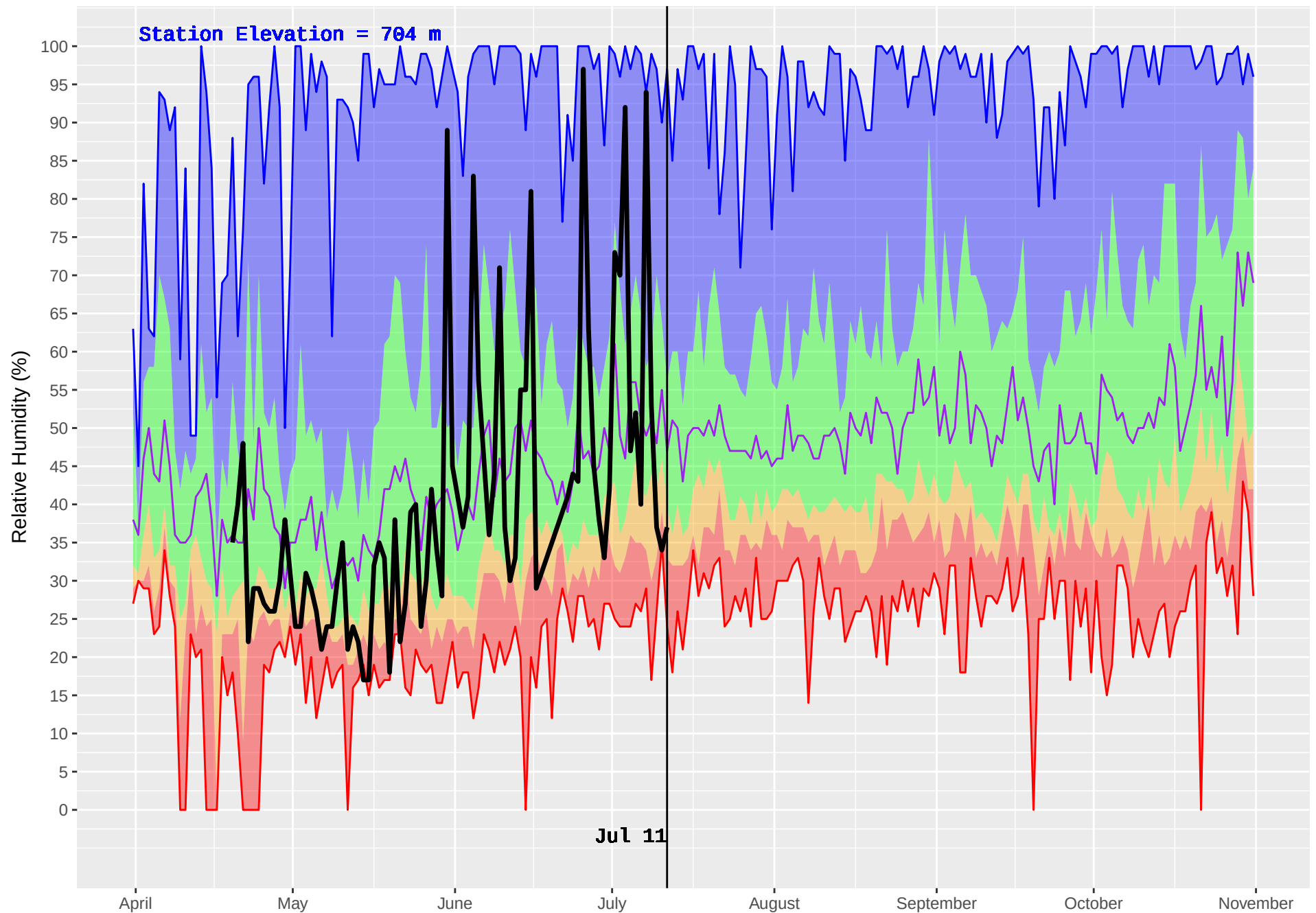
HUDSON HOPE (132) : Historical (1986–2016) and Current (2018) Noon Relative Humidity
