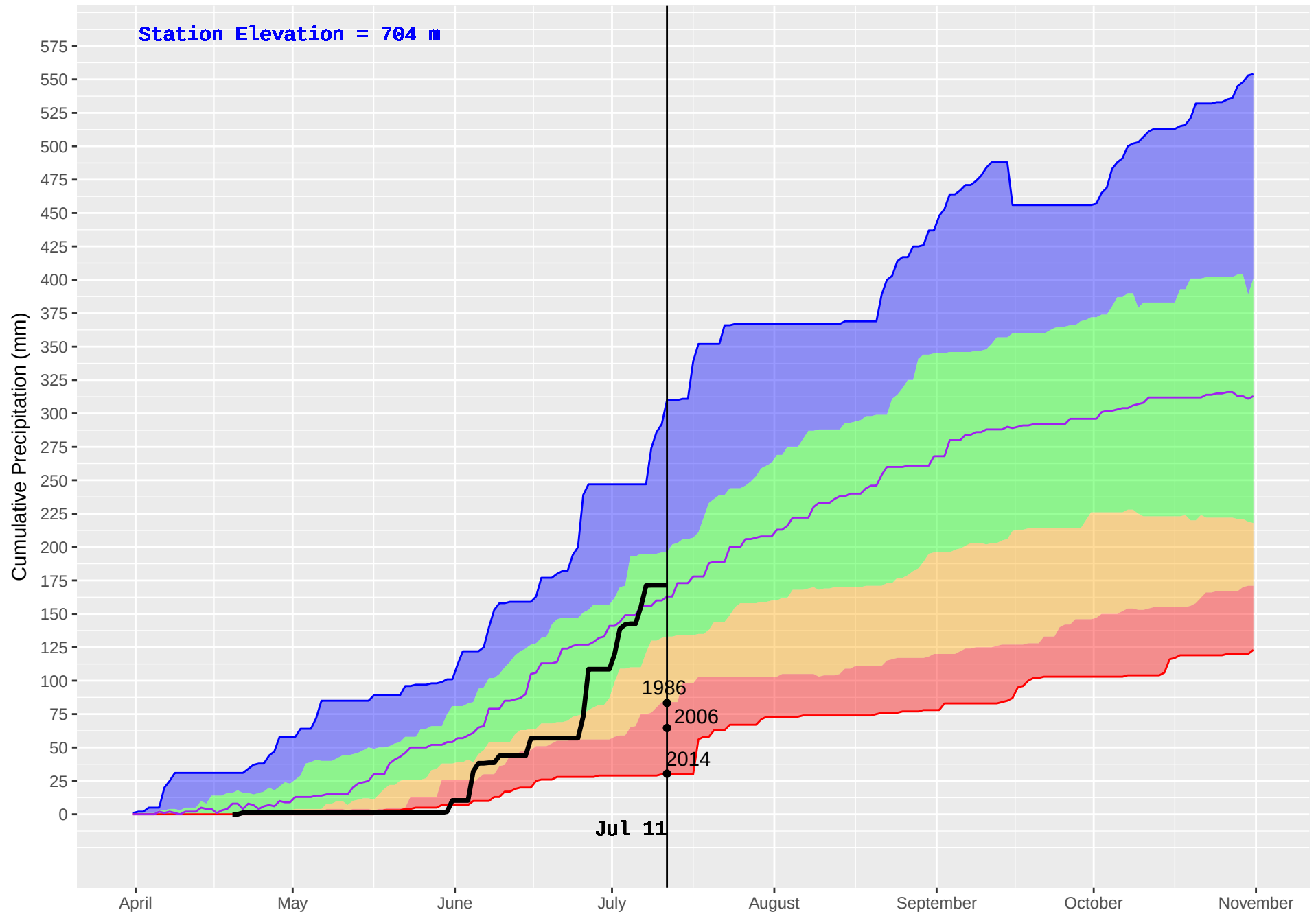
HUDSON HOPE (132) : Historical (1986–2016) and Current (2018) Noon Cumulative Precipitation
