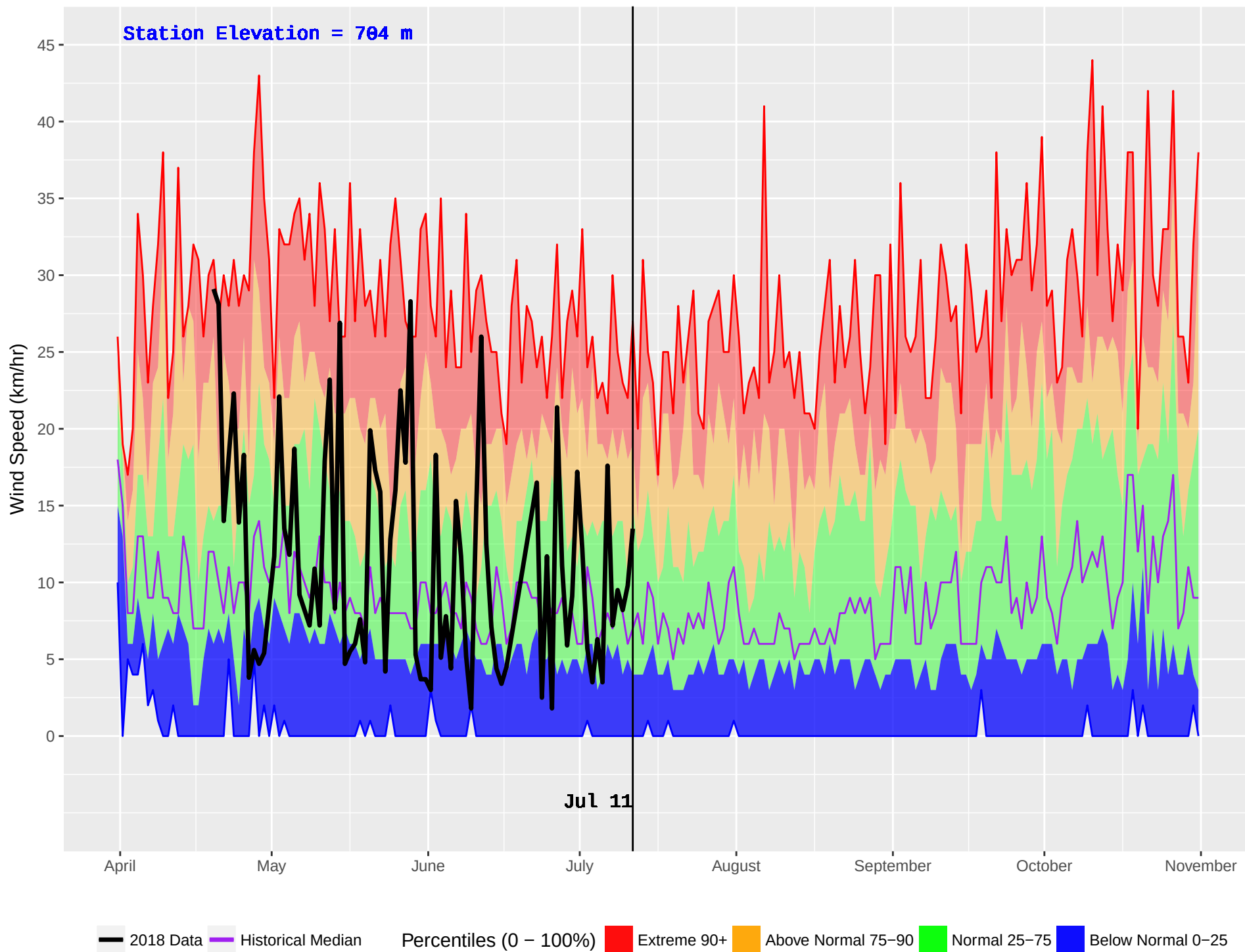
HUDSON HOPE (132) : Historical (1986–2016) and Current (2018) Noon Wind Speed
