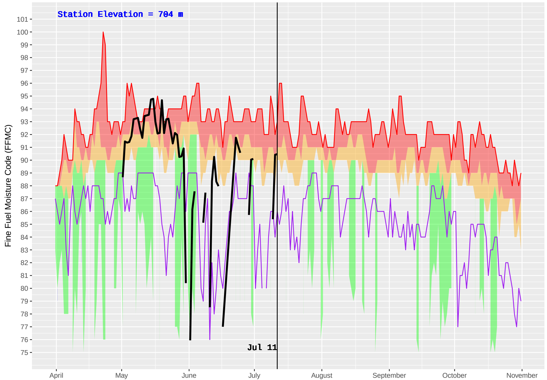
HUDSON HOPE (132) : Historical (1986–2016) and Current (2018) Noon Fine Fuel Moisture Code (FFMC)
