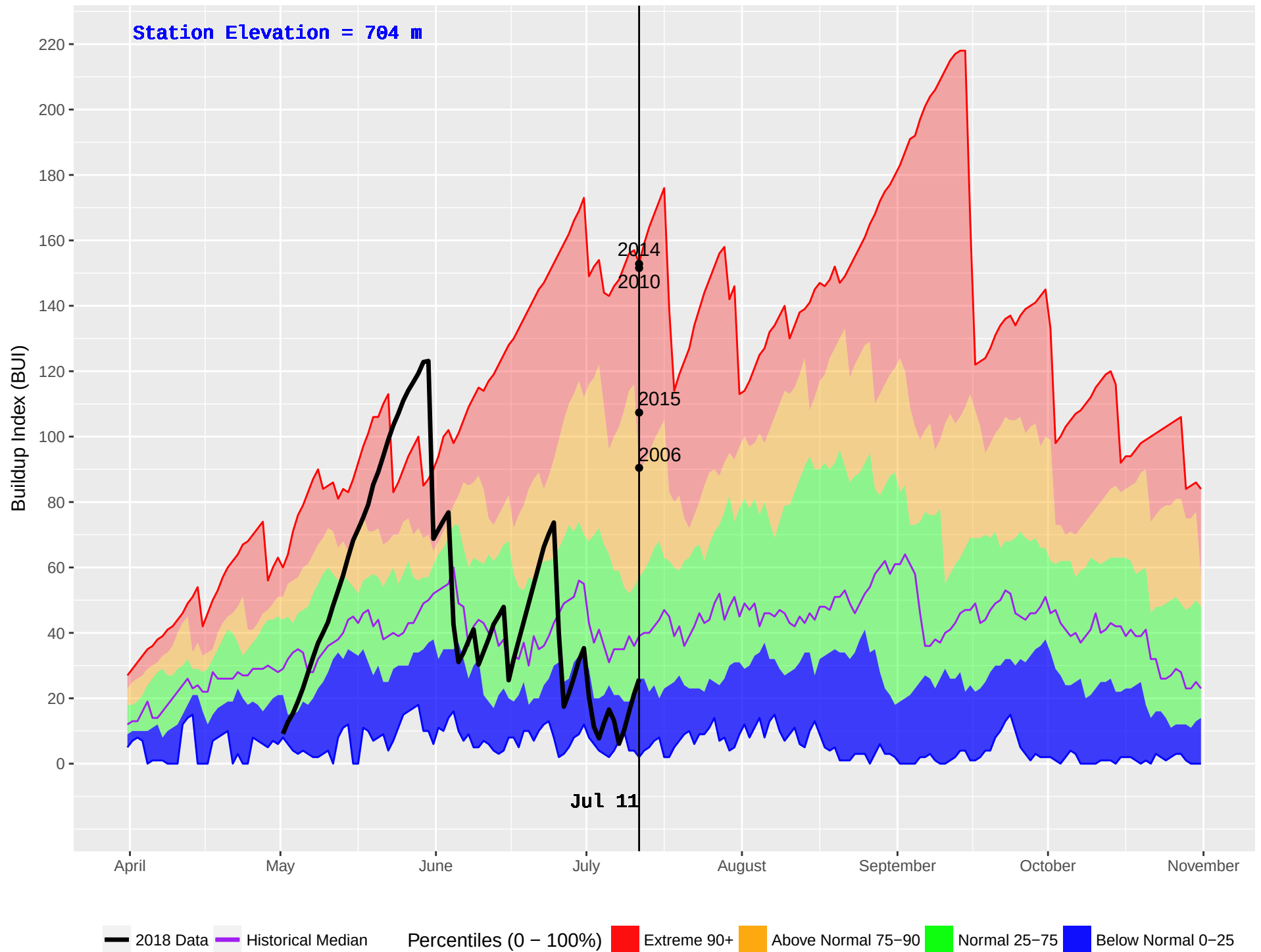
HUDSON HOPE (132) : Historical (1986–2016) and Current (2018) Noon Buildup Index (BUI)
