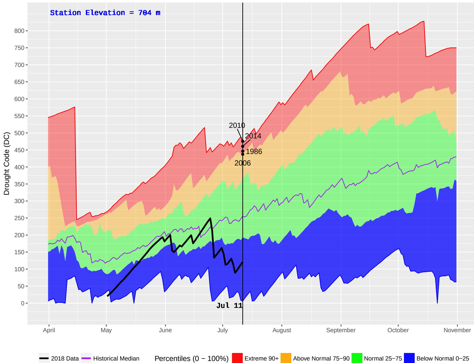
HUDSON HOPE (132) : Historical (1986–2016) and Current (2018) Noon Drought Code (DC)
