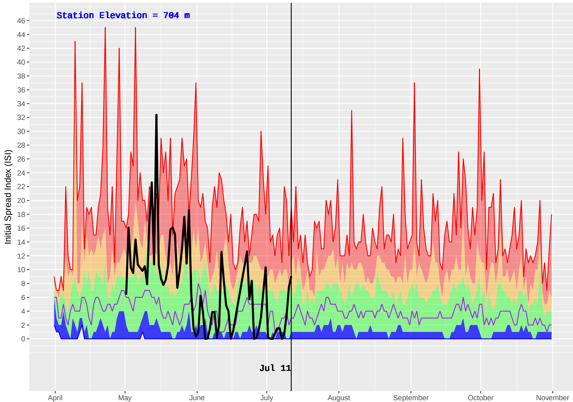
HUDSON HOPE (132) : Historical (1986–2016) and Current (2018) Noon Initial Spread Index (ISI)
