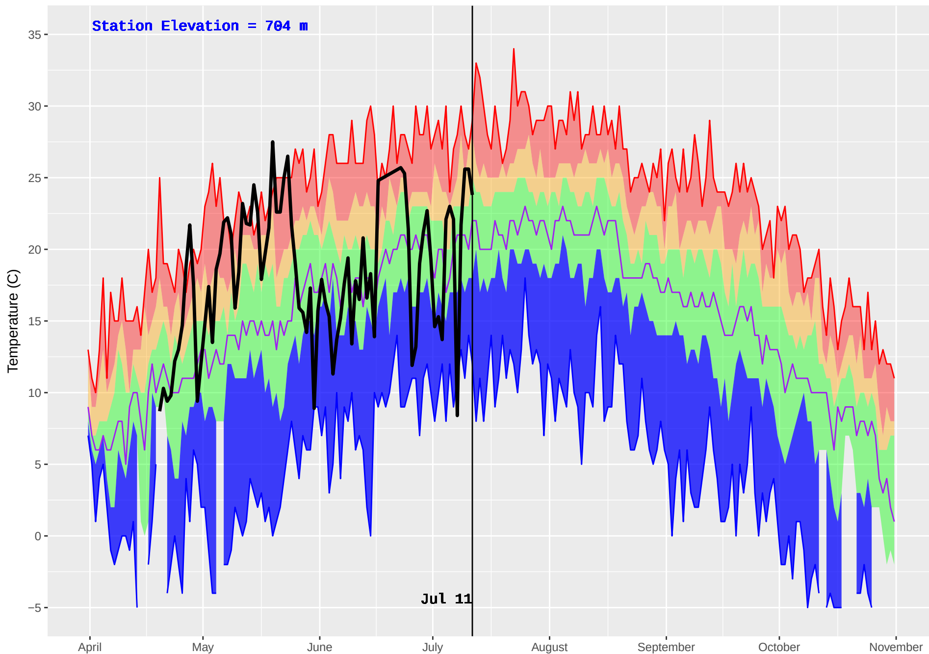
HUDSON HOPE (132) : Historical (1986–2016) and Current (2018) Noon Temperature
