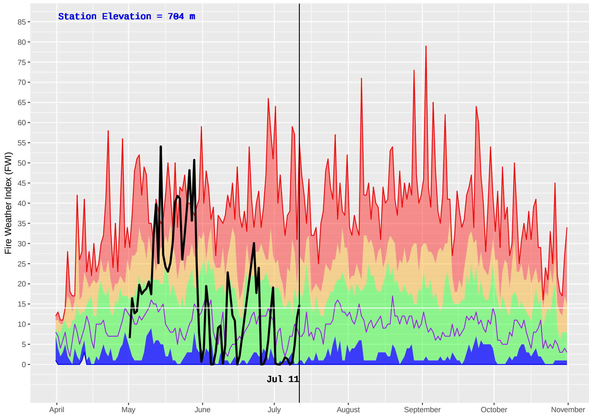
HUDSON HOPE (132) : Historical (1986–2016) and Current (2018) Noon Fire Weather Index (FWI)
